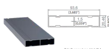
ÜÇLÜ YAN RAY PROFİLİ THREE RAIL SIDE PROFILE
