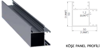
KÖŞE PANEL PROFİLİ CORNER PANEL PROFILE
