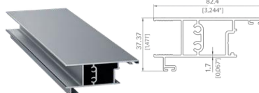
SABİT CAM YAN KİLİT PROFİLİ FIXED GLASS SIDE LOCK PROFILE
