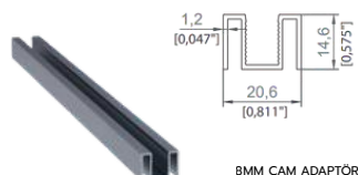
8MM CAM ADAPTÖRÜ 8MM GLASS ADAPTER
