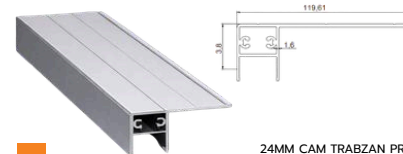
24MM CAM TRABZAN PROFİLİ 24MM GLASS HANDRAIL PROFILE
