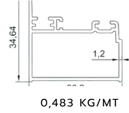
YAN DİKME PROFİLİ SIDE VERTICAL PROFILE
