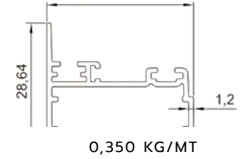
ARA ÇITA PROFİLİ INTERMEDIATE MULLION PROFILE
