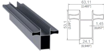
KULPLU PANEL PROFİLİ GLASS PANEL HANDLE PROFILE
