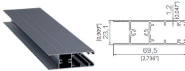
CAM PANEL ALT VE ÜST PROFİLERİ GLASS PANEL BOTTOM AND TOP PROFILES
