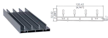
DÖRTLÜ ALT RAY PROFİLİ FOUR RAIL BOTTOM PROFILE
