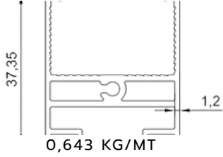
CAM BAZA PROFİLİ GLASS BASE PROFILE
