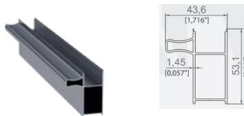
TEK KULPLU PANEL PROFİLİ GLASS PANEL SINGLE HANDLE PROFILE
