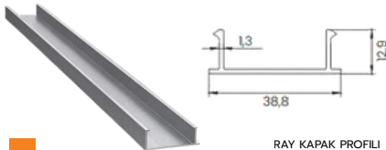
RAY KAPAK PROFİLİ RAIL COVER PROFILE
