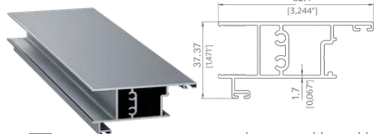
SABİT CAM YAN KİLİT PROFİLİ FIXED GLASS SIDE LOCK PROFILE
