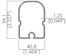
40,8x59,1 İnce Korniş 40,8x59,1 Fabric Support Profile
