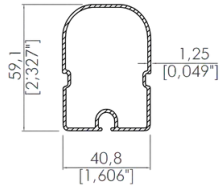
40,8x59,1 İnce Korniş 40,8x59,1 Fabric Support Profile
