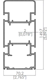
70x150 Ray 70x150 Rail Profile
