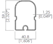
40,8x59,1 İnce Korniş 40,8x59,1 Fabric Support Profile
