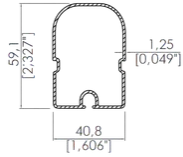
40,8x59,1 İnce Korniş 40,8x59,1 Fabric Support Profile
